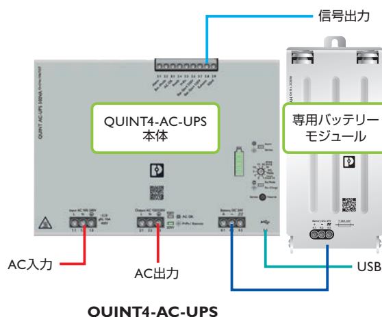
QUINT4-AC-UPS
